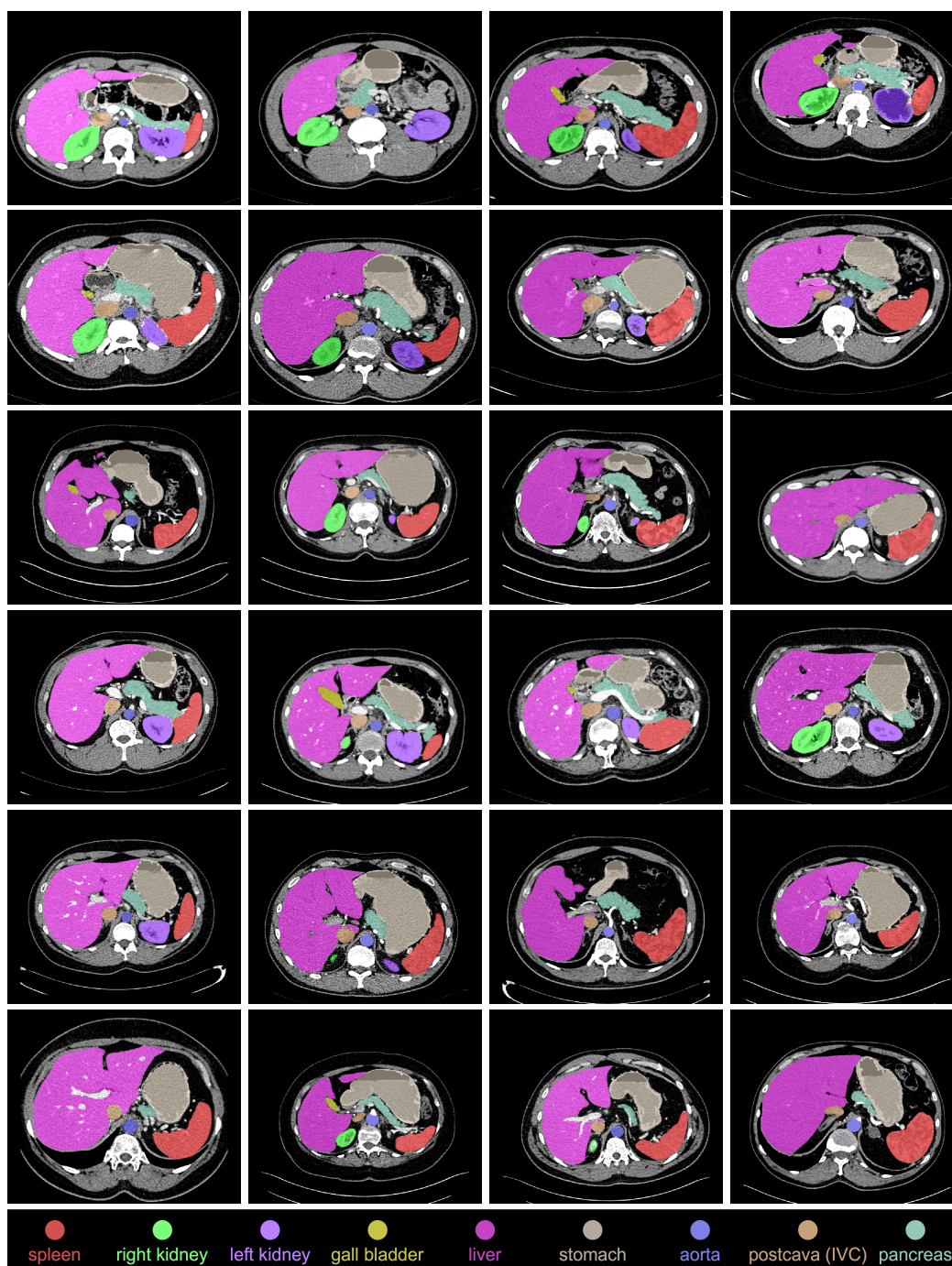
Figure 12: [Watch the animations by clicking them, better viewed with Acrobat/Foxit Reader] Example annotated slices from AbdomenAtlas-8K. AbdomenAtlas-8K includes annotations for eight organs, treating the left and right kidneys as a single organ.
