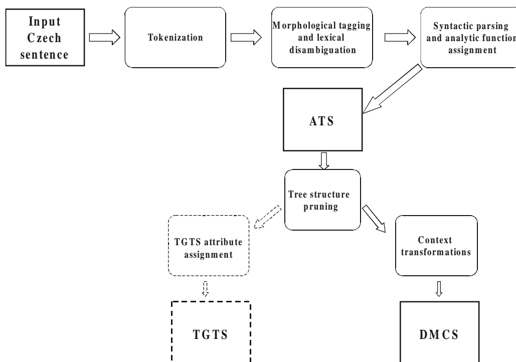
Figure 1: The sequence of procedures in the analysis of a Czech sentence.
