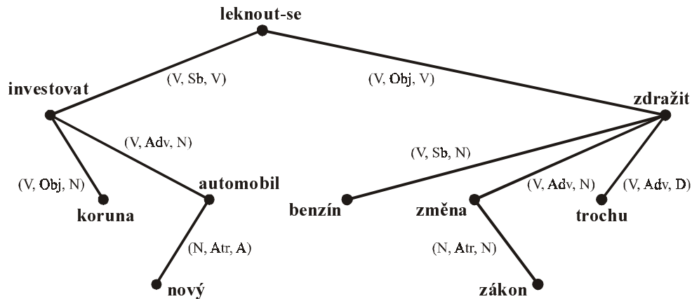
Figure 5: The DMCS of the sentence from Figure 3.
