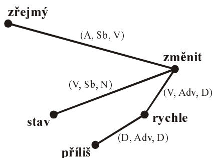
Figure 4: The DMCS of the sentence from Figure 2.
