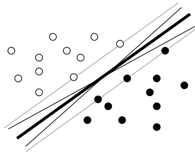
Figure 1: Separating hyperplanes (the set of solid lines), optimal separating hyperplane (the bold solid line), and support vectors (data points on the dashed lines). The dashed lines identify the max margin.
