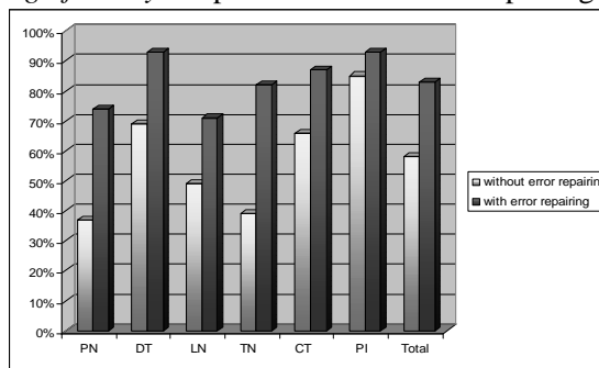
Figure 4: Recall comparison
