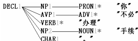
Figure 6. Parse tree of (4)
