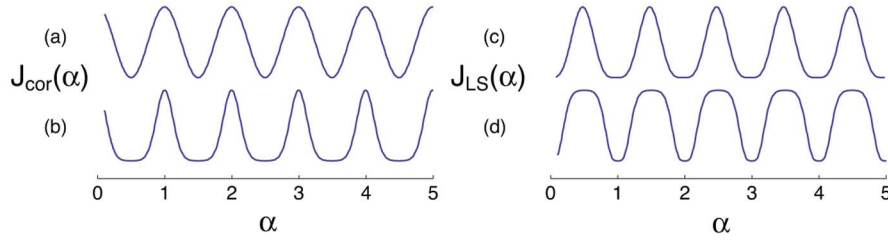
Fig. 5. Cost surfaces for the adaptive phase-reset oscillator. In all four cases, (Gaussian and cosine wave shapes, least squares, and correlation costs) the \alpha parameter is optimized at the “correct” value of 1, or at a simple integer multiple.
