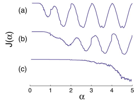
Fig. 9. The cost function for the adaptive phase-reset oscillator when: (a) the input is subjected to additive Gaussian noise with standard deviation 0.004; (b) with standard deviation 0.01; and (c) with standard deviation 0.1. As the amount of noise increases, the optimal values cease to be maxima of the cost function and the oscillator cannot be expected to converge.
