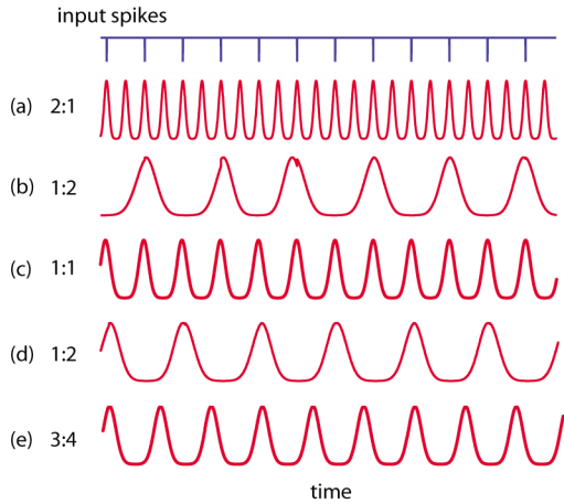
Fig. 3. The input spike train (12) excites the AWO and the parameters \beta and \alpha are updated according to (10) and (11). The initial value in (a) was \alpha = 240 ms and the oscillator synchronizes to a 2:1 rate (two oscillator pulses occur for each input spike). (b) and (d) were initialized at \alpha = 1050 ms. The oscillator synchronizes to a 1:2 rate (one oscillator output for every two input spikes). Depending on the initial value of \beta , the oscillator can lock onto either the odd or the even spikes. (c) was initialized at \alpha = 550 ms. Other synchronizations such as 3:4 are also possible.
