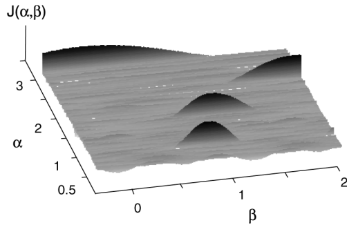
Fig. 10. The cost surface for the phase and frequency updates (10)–(11) of the AWO using the Gaussian wave shape. Additive noise with standard deviation of 0.04 is added to the input, which is a regular train of spikes. Depending on the initial values, the period may converge to \alpha = 1, 2, 3, \dots
