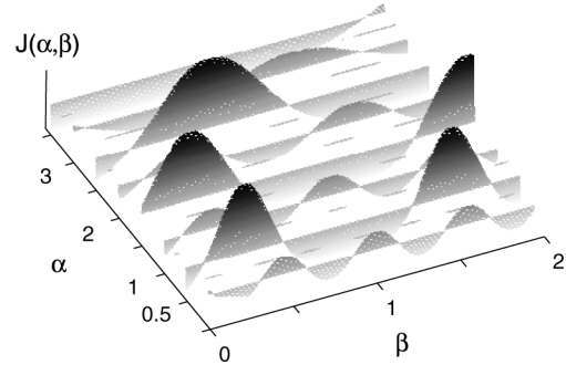
Fig. 6. The cost surface for the phase and frequency updates (10)–(11) of the AWO. Depending on the initial values, the period may converge to \alpha = 1, 2, 3, \dots or any of the other peaks at integer multiples. There are also stable regions of attraction surrounding \alpha = 0.5, 1.5, 2.5, and 3.5 , which correspond to various n:m synchronizations.
