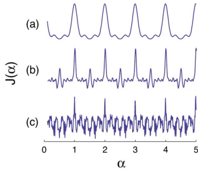
Fig. 7. The cost functions for the adaptive phase-reset oscillator when (a) 50% of the input spikes have been (randomly) deleted; (b) 80% have been deleted; and (c) 95% have been deleted. Despite the high percentages, all still retain their optima at \alpha = n for integers n . As the number of deletions increases, the region of attraction of the optimal values shrinks and local maxima occur.
