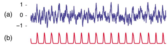
Fig. 11. Changing the input to a train of Gaussian pulses allows the AWO to tolerate additive disturbances, shown here as additive white Gaussian noise with a standard deviation of 0.04.
