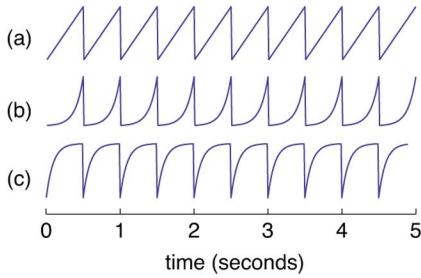
Fig. 1. The trajectories of three phase-reset oscillators. (a) Ramp oscillator with a = 1 , \tau = 1 , b = 0.002 , y_0 = 0 . (b) Growth oscillator with a = 1.1 , \tau = 1 , b = 0 , y_0 = 0.0085 . (c) Decay oscillator with a = 0.9 , \tau = 1 , b = 0.1 , y_0 = 0 .
