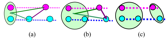
Figure 8: Three stages of the unification algorithm. Green bubbles represent unified clusters.
