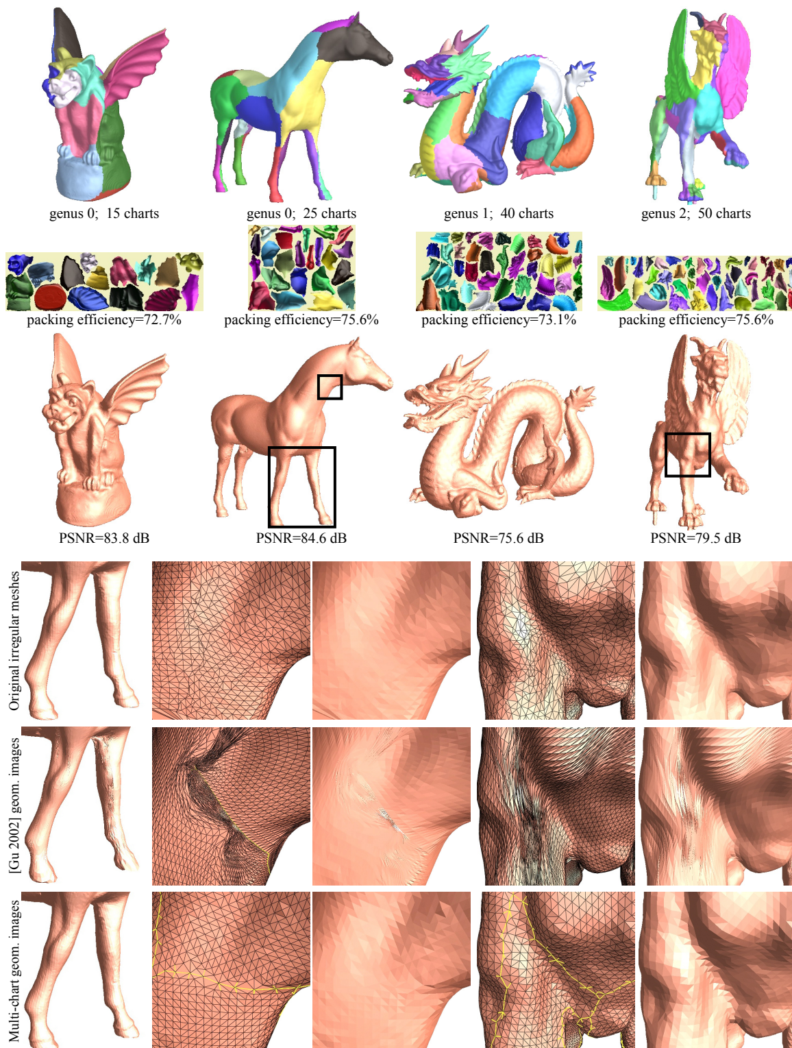
Figure 14: Multi-chart geometry image results. Black squares indicate close-up views used in comparisons below.
