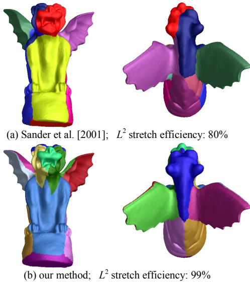
Figure 2: Comparison of the chartification algorithm from Sander et al. [2001] with our new approach on a 12-chart gargoyles. (Garland et al. [2001] would produce results comparable to (a).)
