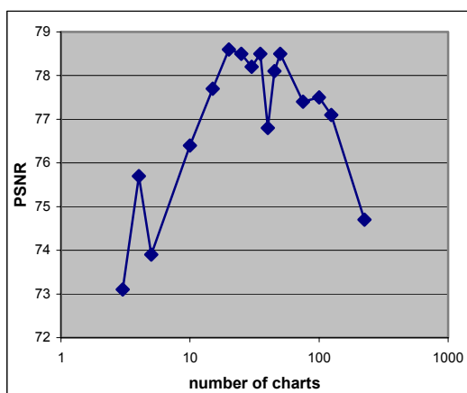
Figure 13: MCGIM accuracy as a function of the number of charts on the horse model, for 128^2 samples.
