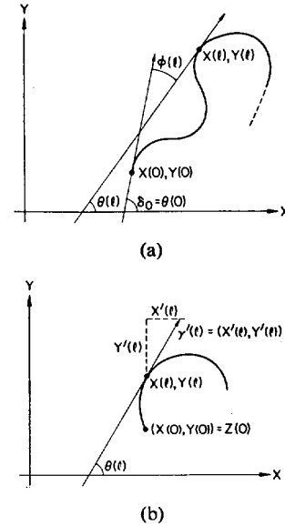
Fig. 1. (a) Parametric representation of a plane curve with tangential direction \theta(l) and cumulative angular bend function \phi(l) . (b) Tangent or velocity vector of plane curve.
