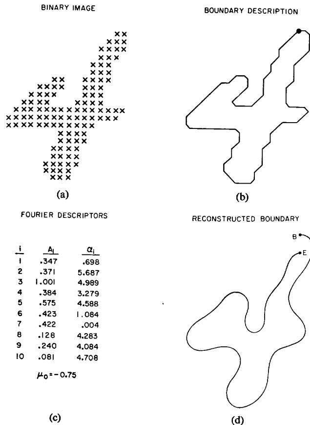
Fig. 5. Fourier descriptor analysis and reconstruction of boundary of a binary image.
