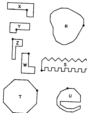
Fig. 4. Simple examples of plane closed polygonal curves.
