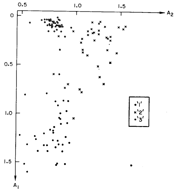
Fig. 6. Clustering of hand-printed characters in the two-dimensional space of the lowest order harmonic amplitudes A_1 and A_2 .
