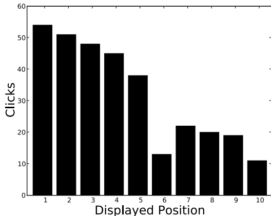
Figure 1: Number of clicks for search operators per display position. Users were twice as likely to click an operator in the first five positions compared to the last five, a strong but weaker bias than for web search where half of all clicks are on the first result and 80% of clicks are on the top 5 [Joachims et al. , 2005]. Our weaker bias may be due to the ease by which users could view other options: operators fit in a small space while web search results require scrolling through sentences.
