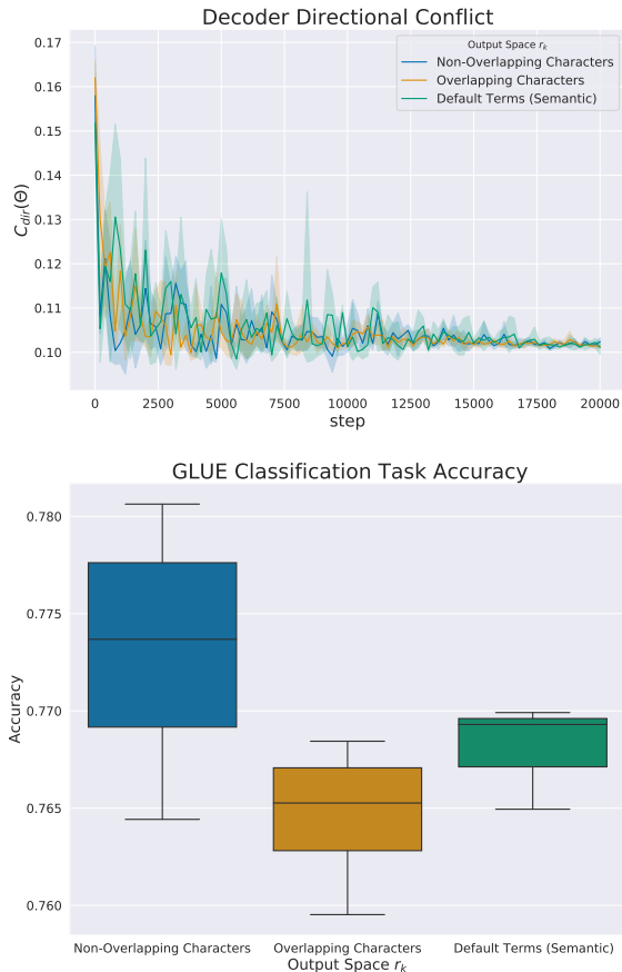
Figure 4: (Top): Directional conflict ( C_{dir} ) in the decoder of GLUE models when using different classification output spaces. The output space used, and the overlap across tasks, has no observable effect on multi-task conflict. (Bottom): The impact of classification output spaces on multi-task performance. Overlap in the output space appears to have an effect on model accuracy: output spaces with less overlap perform better.
