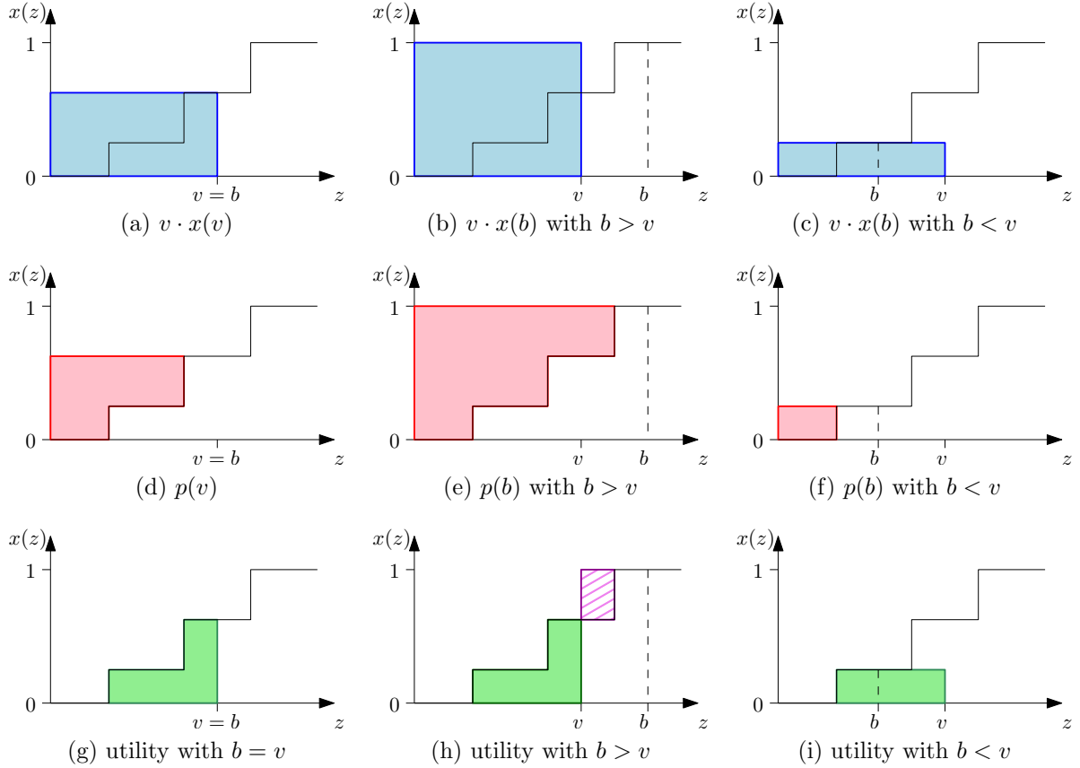
Figure 16.3.2: Proof by picture that (\mathbf{x}, \mathbf{p}) is incentive-compatible
