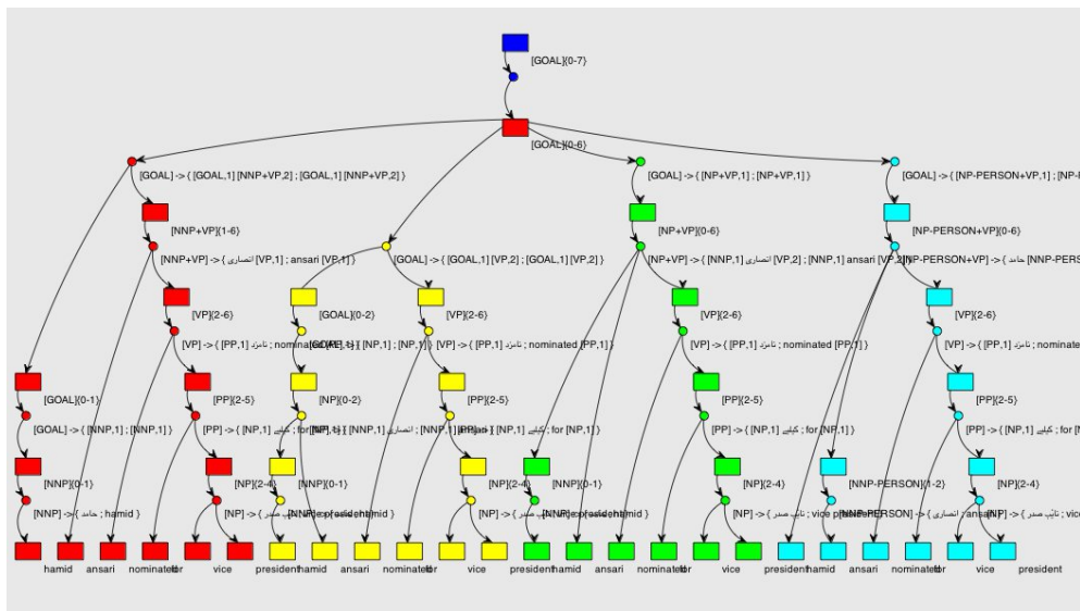
Figure 4. The visualization window for the hypergraph browser.
