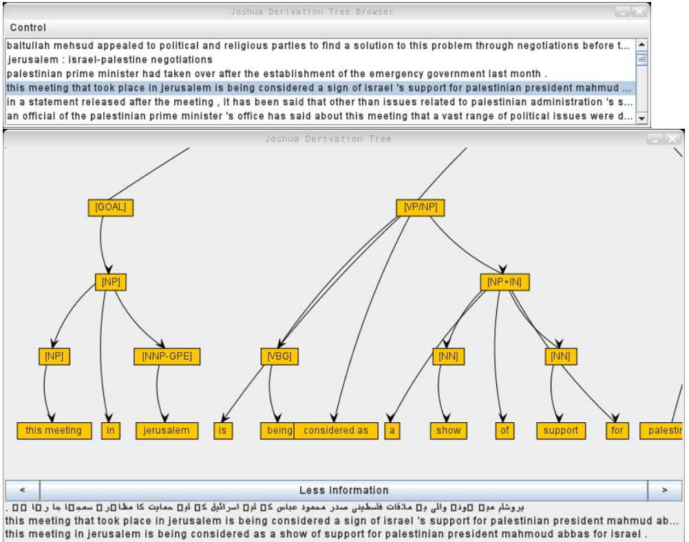
Figure 2. The Derivation Tree browser's sentence selection and tree-viewing windows.
