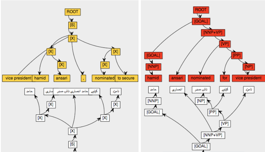
Figure 3. An example visualization of two derivation trees for SCFGs that use a Hiero-style grammar and a syntactically-motivated grammar.
