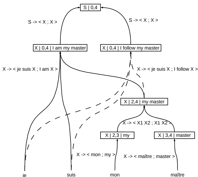
Figure 1. A hypergraph showing two candidate translations of Je suis mon maître .
