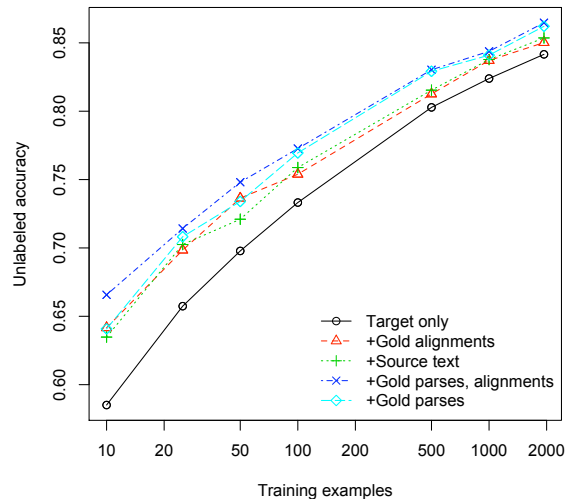
Figure 3: Parser projection with target trees. Using the true or 1-best parse trees in the source language is equivalent to having twice as much data in the target language. Note that the penalty for using automatic alignments instead of gold alignments is negligible; in fact, using Source text alone is often higher than +Gold alignments . Using gold source trees, however, significantly outperforms using 1-best source trees.
