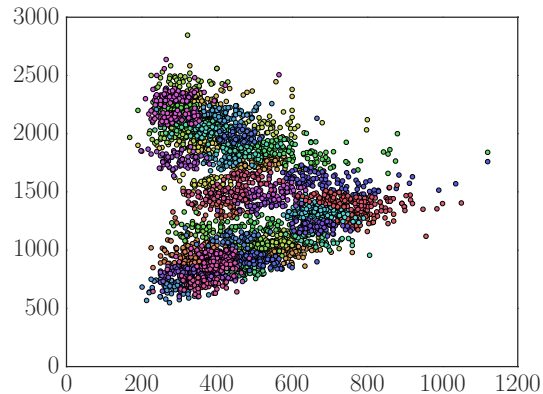
Figure 3: A graph of \mathbf{v} = (F_1, F_2) in the union of all the training languages’ inventories, color-coded by inferred phone ( N = 50 ).
