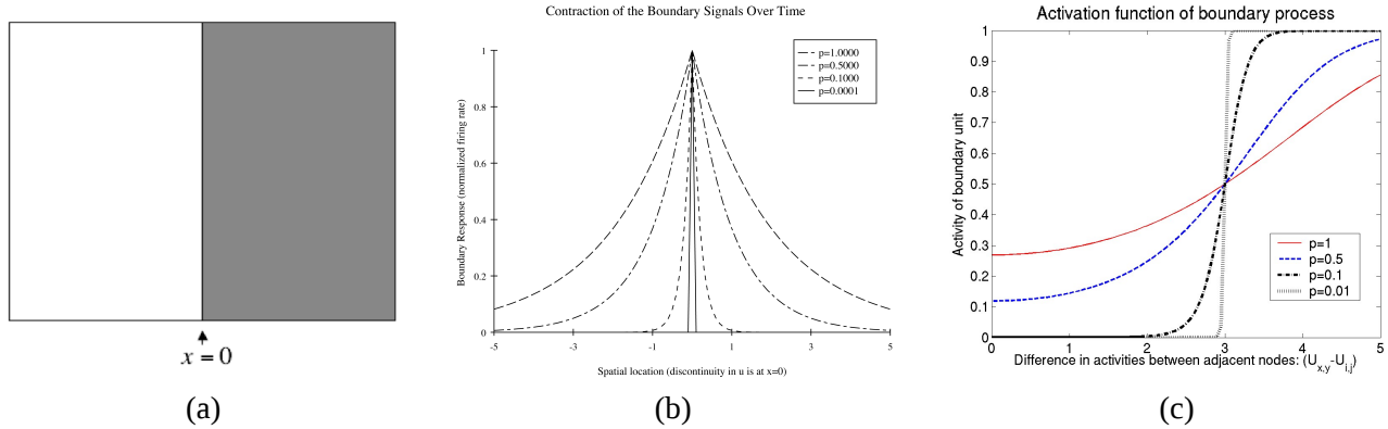
Figure 5: (a) An image with a luminance step edge. (b) In response to the step edge, initially, line processes near the edge will respond, resulting in a broader spatial response profile among these population of nodes. Over time, as p decreases, the boundary responses start to contract spatially to the exact location of the step edge. The activity at each location represents the response of a line process at that location. The curve does represents the responses of a population of identical boundary processors distributed over space, or equivalently the spatial response profile of a boundary unit to different part of the image with a step edge. As p decreases, the spatial response envelope becomes narrower and narrower (Lee 1995). (c) Another perspective on the continuation method is that the activation function of the line process becomes steeper as p decreases (Geiger and Yuille 1991).
