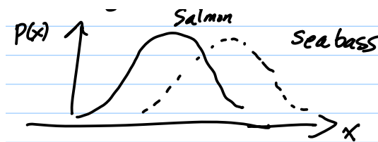
FIGURE 1. Gaussian distributions for the lengths of Salmon and Sea Bass.
