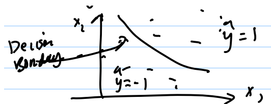
FIGURE 4. Decision boundary is a curve (a quadratic) if the distributions P(\vec{x}|y) are both Gaussians with different covariances.
