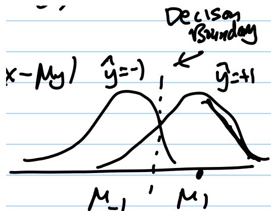
FIGURE 2. Decision boundary for Salmon and Sea Bass.
