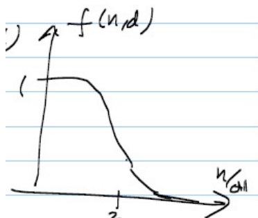
FIGURE 5. Plot the function f(n, d) as a function of n/(d+1) . For small n < d+1 the value is 1. For n \gg 2(d+1) the value is almost 0, so there is also no chance that we can find a separating plane by 'luck'. If we find a separating plane, then it probably corresponds to structure in the data and will enable us to generalize.
