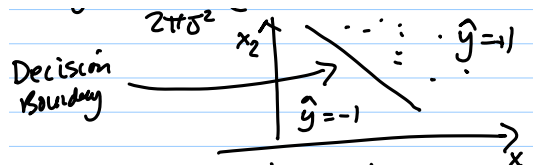
FIGURE 3. Decision boundary is a line if the distributions P(\vec{x}|y) are both Gaussians with the same covariance \sigma^2 (times identity matrix).
