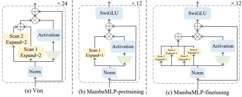
Figure 4: The comparison of block architectures between Vim, and MambaMLP in pretraining and in finetuning.
