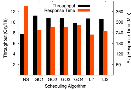
Figure 14: Throughput and response time by algorithm.
