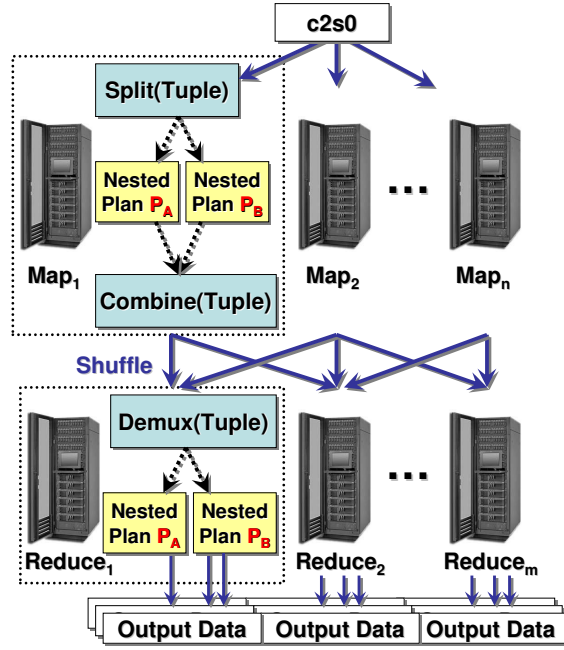
Figure 3: Nested execution of Pig program P_{AB} .
