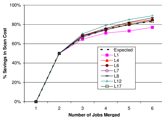
Figure 10: Actual vs estimated savings in scan cost.
