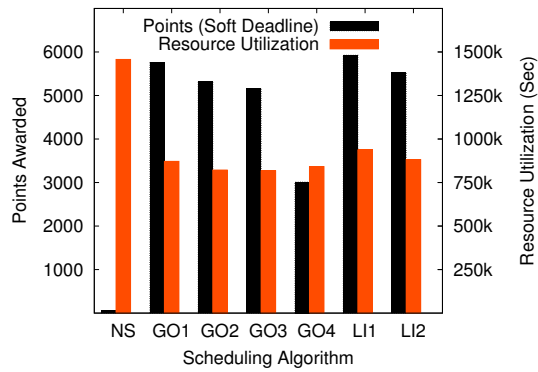
Figure 12: Points awarded and resource usage by algorithm.
