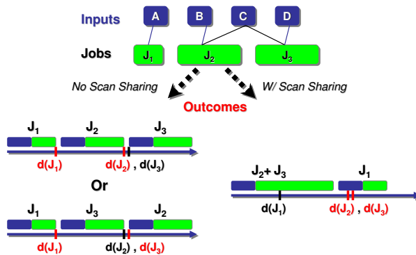
Figure 4: Scheduling outcomes (with and without scan sharing). Deadlines met are shown in red.
