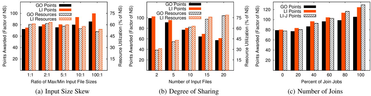
Figure 15: Sensitivity of GO and LI algorithms to workload changes.
