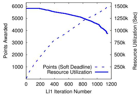
Figure 13: Best schedule over time for local improvement (LI).
