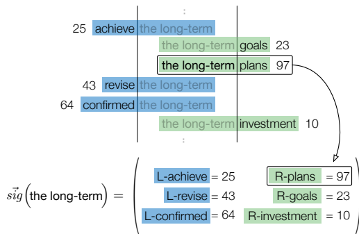
(a) The n -gram corpus records the long-term as preceded by revise (43 times), and followed by plans (97 times). We add corresponding features to the phrase’s distributional signature retaining the counts of the original n -grams.
