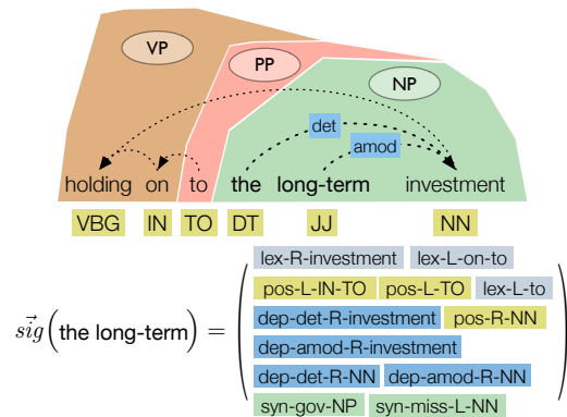
(b) Here, position-aware lexical and part-of-speech n -gram features, labeled dependency links, and features reflecting the phrase’s CCG-style label NP/NN are included in the context vector.
