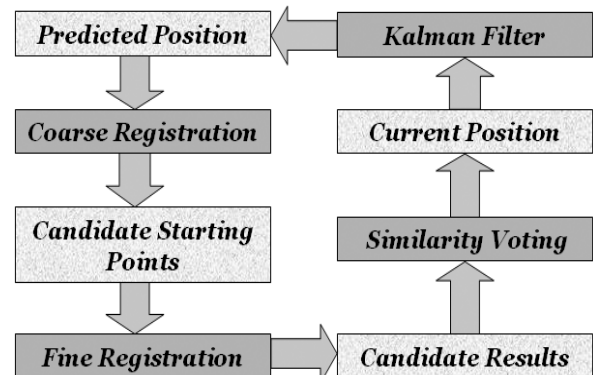
Fig.3 Algorithm framework
