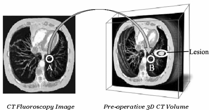
Fig.2 Local registration
