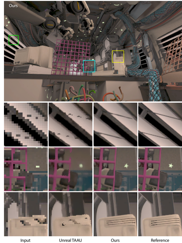
Fig. 6. Comparison with Unreal TAAU with 4 \times 4 supersampling. The PSNR and SSIM of our and TAAU results are computed with respect to each’s own reference image rendered at Unity and Unreal respectively. Our resulting PSNR is 31.74dB, SSIM is 0.9430, outperforming TAAU whose resulting PSNR is 30.06dB, SSIM is 0.9070.
