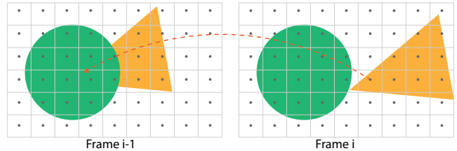
Fig. 3. Illustration of the subpixel backward motion vector rendered by game engines. The rendered point samples are represented by the black circle points at the center of each pixel. An example of the subpixel backward motion vector between frame i and i - 1 is illustrated by the red dashed line. The motion vector defines where an infinitesimal 3D point that is visible at frame i would appear at its previous frame i - 1 , without its visibility or color information.
