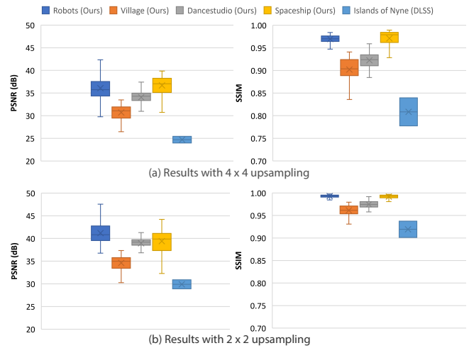
Fig. 11. Discussion figure for DLSS quality. The content for DLSS and for our method is different, and we were able to capture only a few pixel accurate image pairs, so a direct comparison is not possible. This plot is meant to illustrate that the quality ballparks for both methods are comparable. Box and whisker chart of the quality for (a) 4 \times 4 upsampling and (b) 2 \times 2 upsampling, by our method and DLSS on different scenes.
