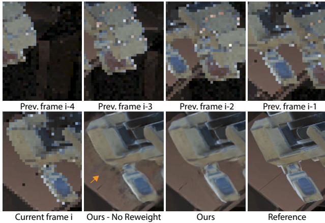
Fig. 10. Ablation experiment for the feature reweighting module. When the network is trained without the reweighting module (“Ours-NoReweight”), ghosting artifacts appear at the disoccluded regions as pointed by the orange arrow.
