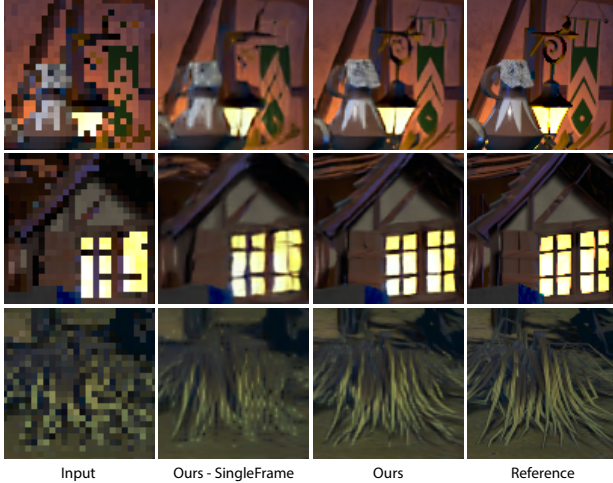
Fig. 9. Ablation experiment for performance gain from using previous frames. “Ours-SingleFrame” represents the trained network that takes only a single frame as input.
