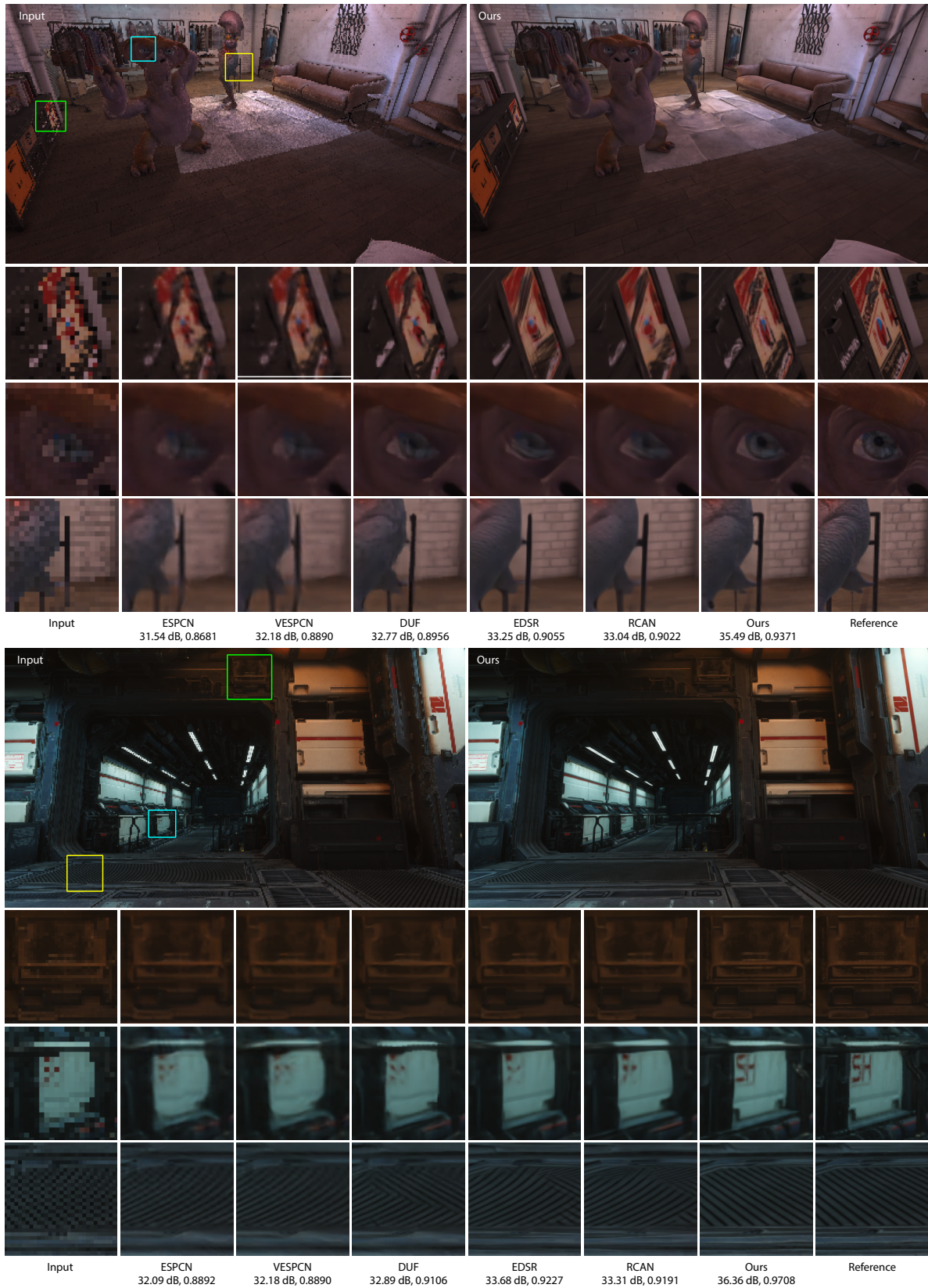
Fig. 8. Visual results on the DanceStudio (top) and Spaceship (bottom) scene. Asset credits to Ruggero Corridori and Unity Technologies respectively.
