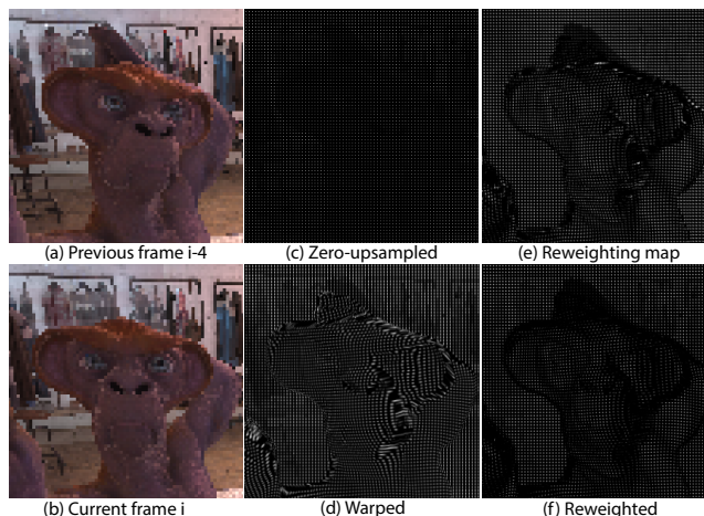
Fig. 5. Example intermediate outputs of our method. In subfigures (c)-(f) we visualize a single channel of the feature map in greyscale. The features of previous frame i - 4 are zero-upsampled (fig. c) and warped to align with the current frame i , using the subpixel backward motion vectors (fig. d). The warped features go through the feature reweighting subnetwork (fig. e), and the re-weighted features (fig. f) are then fed into the reconstruction subnetwork for final results. Best viewed zoomed on a monitor.
