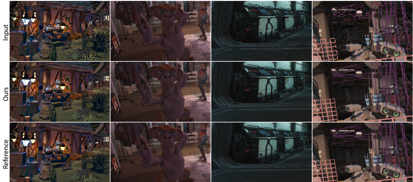
Fig. 1. Results of our real-time, learned 4 \times 4 supersampling are shown for four sample scenes. From top to bottom: the rendered low-resolution color input, our reconstruction, and the rendered reference images. Our supersampling method takes the color, depth, and motion vectors of multiple low-resolution frames, and produces high-fidelity reconstructions by reducing aliasing and recovering scene details.
