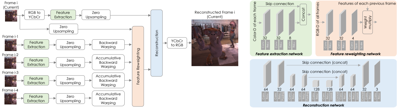
Fig. 4. Network architecture of our method. Left shows an outline of the method and right shows the architecture of each sub-network, including the feature extraction, feature reweighting, and reconstruction networks. The numbers under each network layer represent the output channels at corresponding layers. The filter size is 3 \times 3 at all layers. The tanh layer in the feature reweighting network is followed by a scaling operation to map the values from (-1, 1) to (0, 10) .
