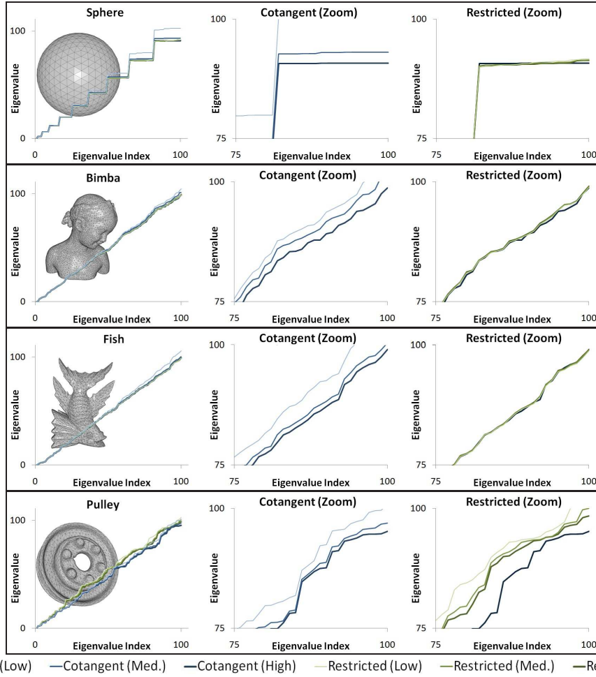
Figure 3: Using our Laplace-Beltrami operator, we compute a spectrum that only depends on the geometry of the surface. In contrast, using the cotangent formulation results in a spectrum sensitive to the tessellation.
