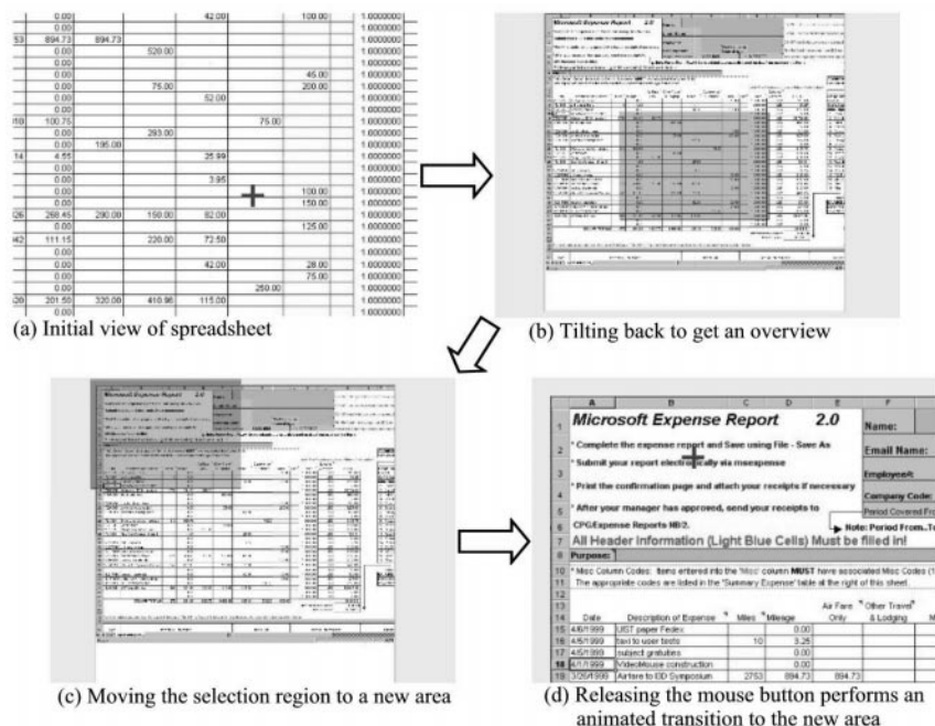
Fig. 7 Several snapshots from a sequence of the user navigating through the spreadsheet.
