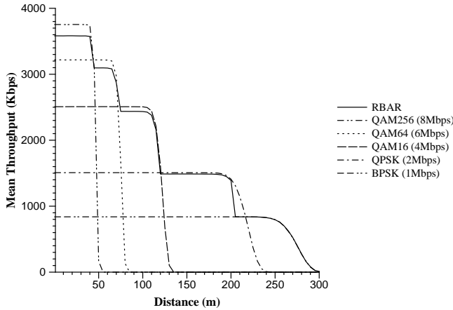
Figure 12: Performance of RBAR for a single CBR connection between two nodes at fixed distances.
