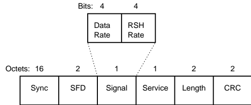
(c) Physical layer (PLCP) header.
