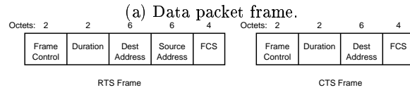
(b) RTS/CTS control packet frames.
