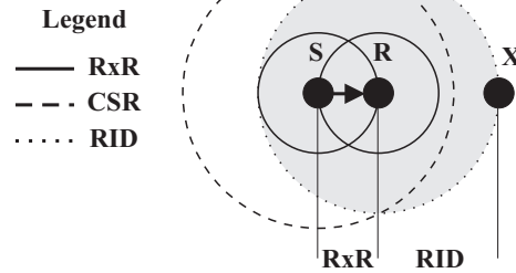
Figure 2. The receiver interference distance ( RID ) is the distance between a receiver ( R ) and another sender ( X ), such that the receiver can successfully receive S 's packets and X can simultaneously send a packet to another receiver.
