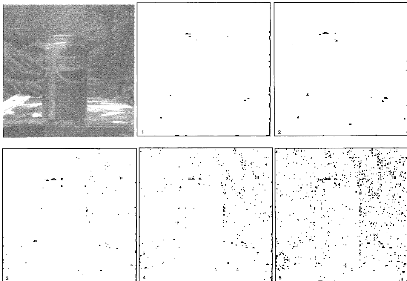
FIG. 18. The Pepsi sequence; data outliers. Results of the continuation method stages 1–5 (see text).
