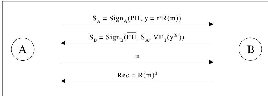
Fig. 1. Off-line certified e-mail protocol via verifiable encryption of RSA signatures
