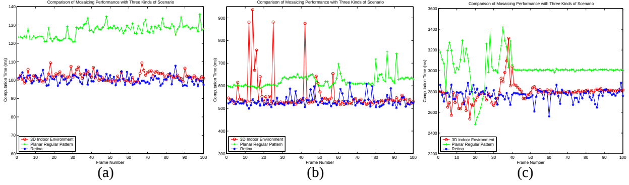
Figure 8: Performance comparison of image registration under different image resolution. (a) 160 \times 120 (b) 320 \times 240 (c) 640 \times 480 .
