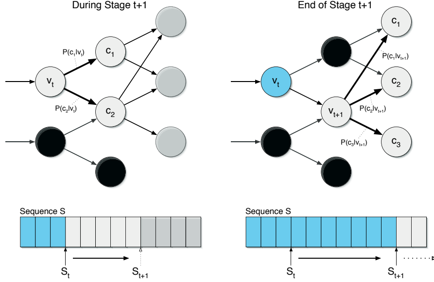
Figure 3 Graphical depiction of two stages of the proposed greedy algorithm for computing the inference on the PGM. Dark gray nodes are not on the best path and are disregarded, and blue represents past objects on the best path.
