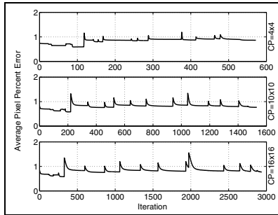
Figure 3: Tracking Convergence.
