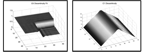
Figure 7: Fitting Discontinuities.
