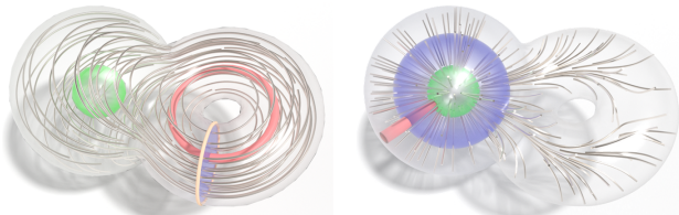
Fig. 7. Absolute and relative homologies. Homology generators and corresponding harmonic fields on a topological torus with a spherical cavity inside. The red loop (left) around tunnel represents the first homology, and the blue membrane is its dual in the second relative homology. The red curve (first relative homology generator, right) is a loop when the boundary is considered as a point, and the blue membrane is its dual in the second homology. Each harmonic field has the same circulation (resp., flux) on all loops (resp., membranes) that can deform into each other in the domain.
