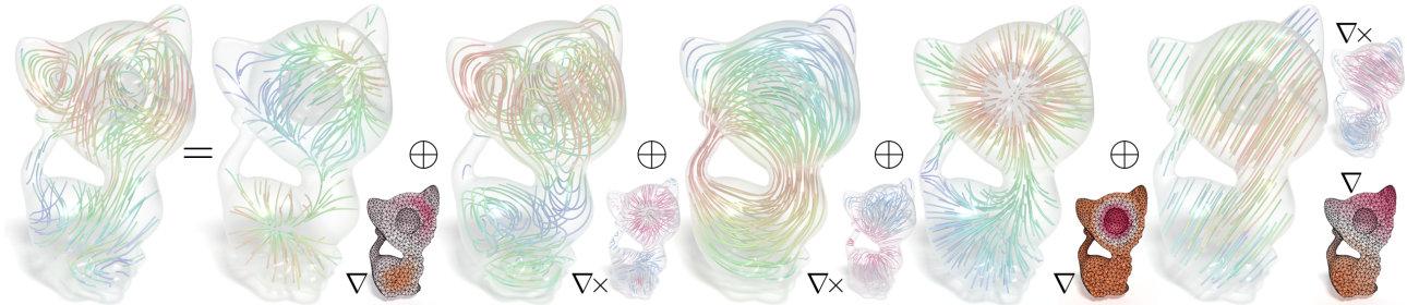
Fig. 1. Five-Component Vector Field Decomposition. On a tetrahedral mesh of the kitten with a spherical cavity, a vector field is decomposed into a gradient field with zero potential on the boundary, a curl field with its vector potential orthogonal to the boundary, a pair of tangential and normal harmonic fields, and a harmonic field that is both a gradient and a curl field. Potential fields are shown in the corners of their corresponding components.
