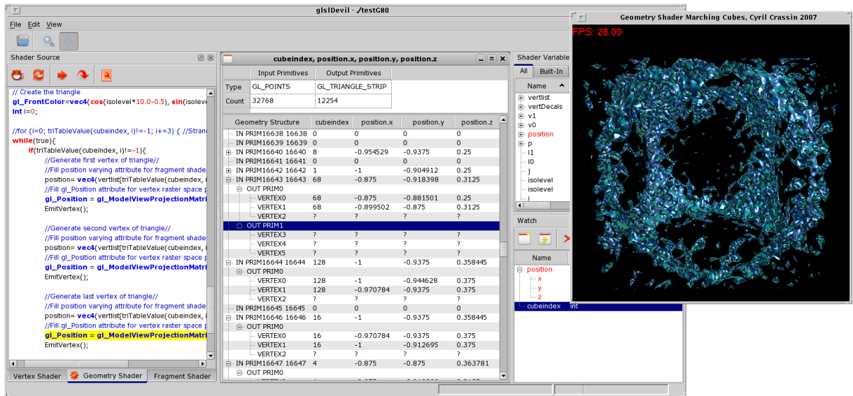
Figure 4: Debugging a geometry shader: Data inspection is performed on a per input primitive level, showing for each input primitive the resulting output primitives and their corresponding vertices. Variable content at the current debug position is shown for each input primitive. Additionally, for already emitted vertices the variable values at the time of emission are shown. Questionmarks indicate output vertices that are not yet emitted.
