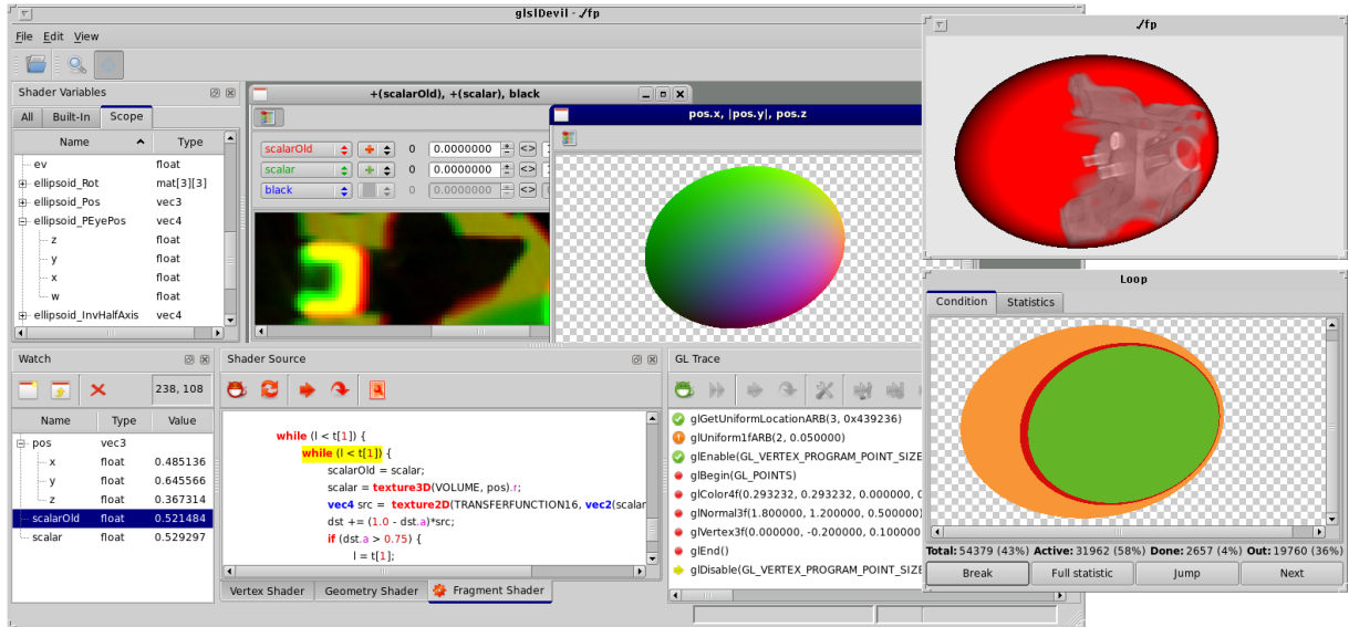
Figure 3: A typical debugging session: From the original application's (top right) OpenGL stream a single draw call is selected and the active fragment shader is debugged having shader source code, scope lists, variable data content, and graphical analysis tools at hand. Status information of the currently debugged loop statement (bottom right) supports the user in program flow decisions.
