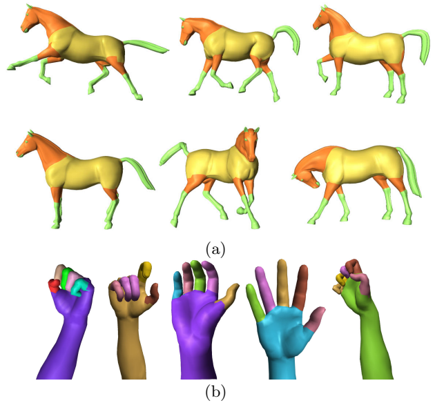
Fig. 9 Despite pose changes, partitioning based on the SDF function remains consistent as can be seen on the horse model (a) and human hand (b).
