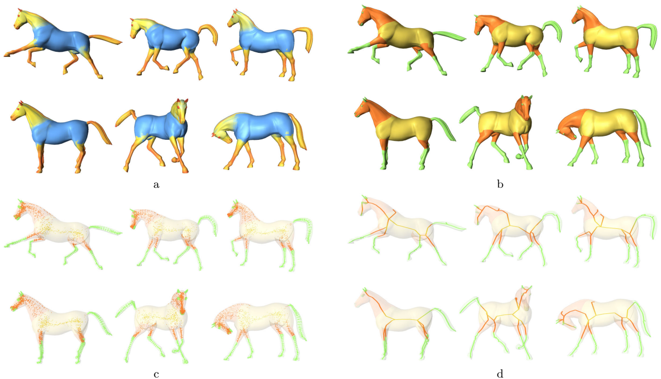
Fig. 15 (a) Consistent SDF on six horses poses (b) Consistent partitioning (c) The projected points retain a strong connection to the surface. Each projected point is colored in its matching face's partitioning color (d) the final consistent skeleton, strongly tied to the surface
