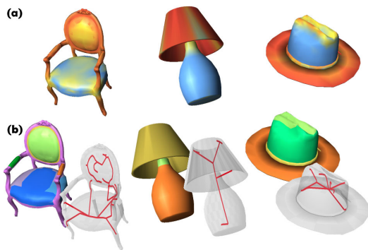
Fig. 16 The SDF value on non-articulated objects (a), and the results of partitioning and skeletonisation on such objects (b)
