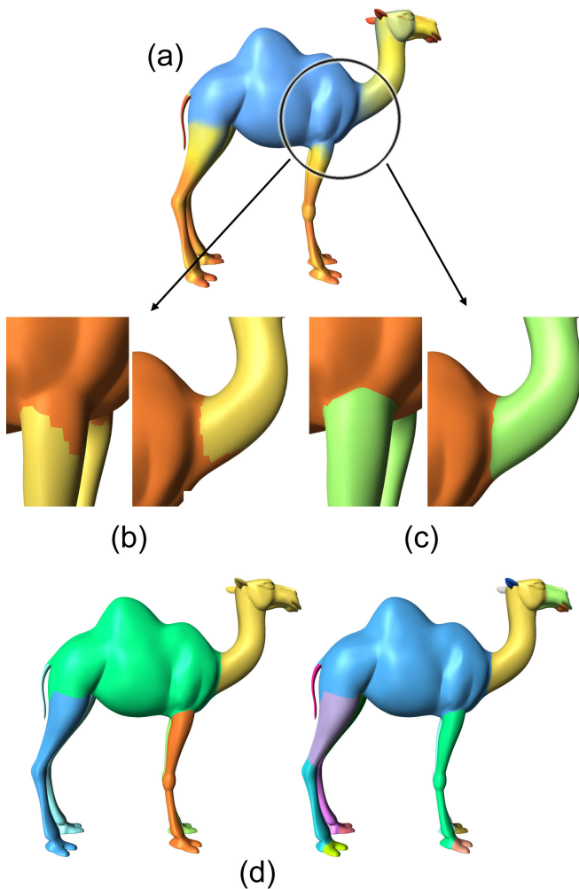
Fig. 8 The two step partitioning algorithm: (a) SDF values are clustered to create soft partitioning of the mesh. (b) After the first step we show the soft partitioning using simple thresholding. (c) The partition is refined by the second step of k-way graph-cut algorithm that creates smooth boundaries and adheres to local features such as concave areas on the mesh. (d) The hierarchical partitioning is robust, pose oblivious and fast.
