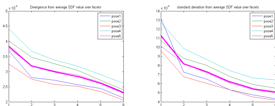
Fig. 5 The effect of enlarging the cone angle and adding more rays on the consistency of the SDF over different poses.
