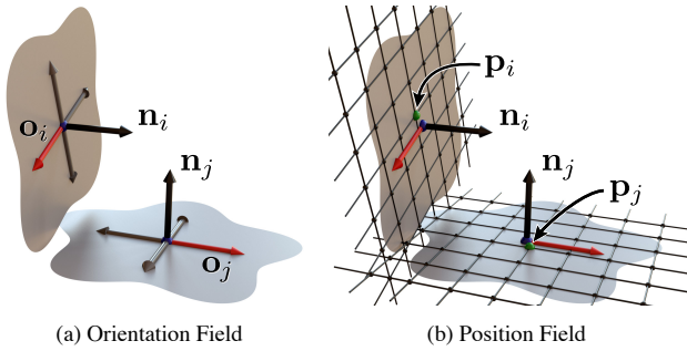
Fig. 2. Illustration of the fields used by the Instant Meshes technique. (a) Neighboring point cloud vertices v_i and v_j representing surface observations (abstract shapes) with normals n_i and n_j store orientations o_i and o_j (red arrows) that control the alignment of the output mesh. The orientations satisfy a rotational symmetry (RoSy) condition, such that each direction is part of an equivalence class with three other elements (grey arrows); a hierarchical optimization scheme optimizes the field smoothness subject to this symmetry. (b) The position field controls the fractional offset (green dot) of a local parameterization (regular grid) that is aligned with the previously computed orientations and used to mesh the point cloud. A similar positional symmetry (PoSy) defines translated versions of the offset (black dots at grid intersections) are equivalent. The position step then optimizes the smoothness of the position field subject to this symmetry.
