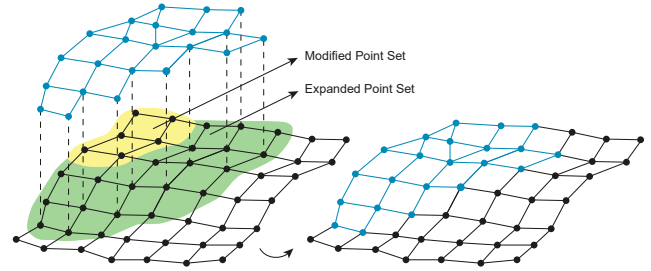
Fig. 8. Coarse mesh update. The set of modified points is grown to yield an expanded point set, from which a partial mesh is extracted. This partial overlay mesh is then integrated into the old mesh, replacing overlapping areas.
