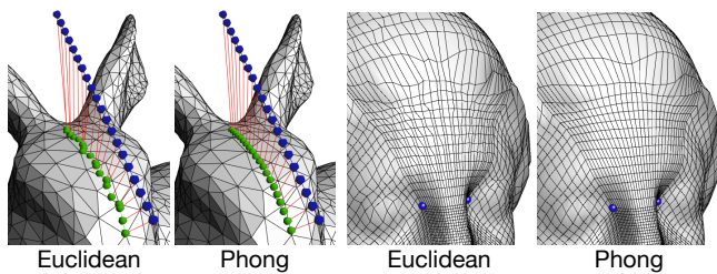
Figure 3: Left: A line segment in 3D space projected onto a mesh using Euclidean and Phong projection. Right: Quad remeshing (see Section 4) using Euclidean and Phong projection in \mathbb{R}^D . Notice the jaggedness of the Euclidean projections.
