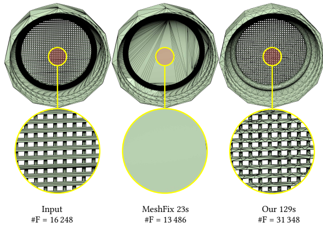
Fig. 19. Example of repairing an invalid triangular mesh (left) with MeshFix (middle) and our algorithm (right). MeshFix is fast but loses details during processing, while our method preserves them. The max AMIPS energy of our intermediate tetrahedral mesh is 1975. Here we stop mesh improvement when maximum energy reaches 2000.
