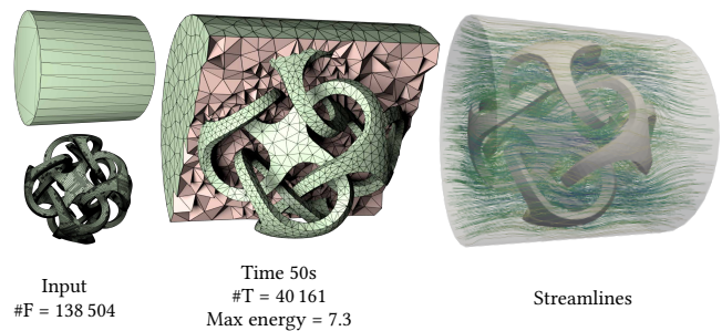
Fig. 27. Streamlines of a fluid (right) moving in a cylindrical pipe (left top) with a complicated obstacle (left bottom) in the center. The background mesh (middle) is obtained by subtracting the obstacle from a cylinder using our method.
