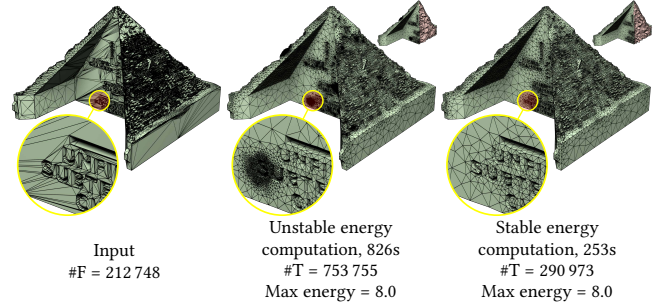
Fig. 10. Example of model where the numerical instability of the AMIPS energy causes over-refinement (middle). By evaluating the energy using rational numbers (when it is above 10^8 ) the issue disappears (right).
