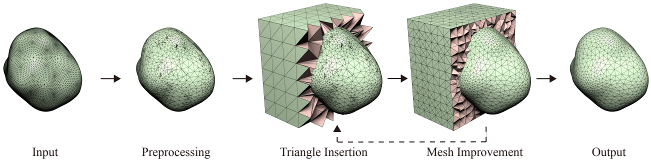
Fig. 3. Overview of our algorithm. From left to right, the input mesh is simplified, a background mesh is created and the input faces are inserted, the mesh quality is optimized, and the final result is obtained by filtering the elements lying outside the input surface.
