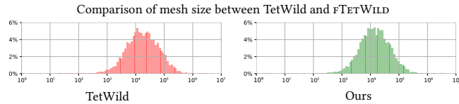
Fig. 18. Histograms of number of tetrahedra in log scale for the output meshes of Thingi10k dataset.
