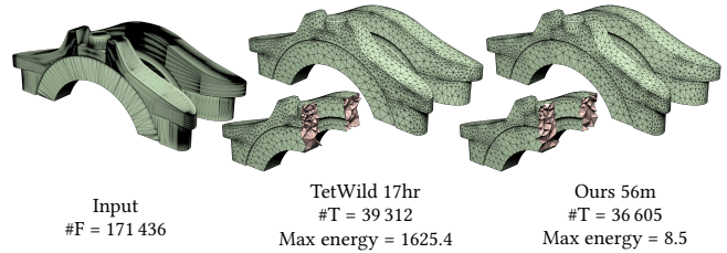
Fig. 15. Example of a challenging model where fTetWild is 17 times faster than TetWild.
