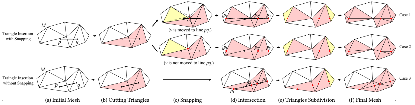
Fig. 5. Segment insertion into a triangle mesh (a 2D analog of triangle insertion) with and without snapping. (a) Insertion of segment pq into mesh M . (b) Identification of cut triangles \mathcal{T}_I (in red). (c) Snapping vertex v to line pq and updating \mathcal{T}_I , where v is \delta -close to pq . v is moved to its closest points on line pq if this does not invert any elements of M (case 1). Vertex v is added in \mathcal{V}_\delta both if v is moved (case 1) or not (case 2). The yellow triangle is added to \mathcal{T}_I . (d) Computing the intersection of line pq with the edges of \mathcal{T}_I (points p_1, p_2, p_3 ). (e) Triangles requiring subdivision (shown in red). (f) The final mesh after subdivision.
