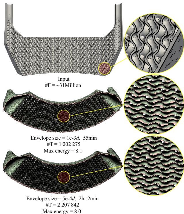
Fig. 21. Meshing a complex model with 93 million vertices and 31 million faces with different envelope sizes (top). The input mesh contains degenerate triangles and severe self-intersections. Our output tetrahedral meshes are in geometric high quality with either default envelope size (middle) or half envelope size (bottom).
