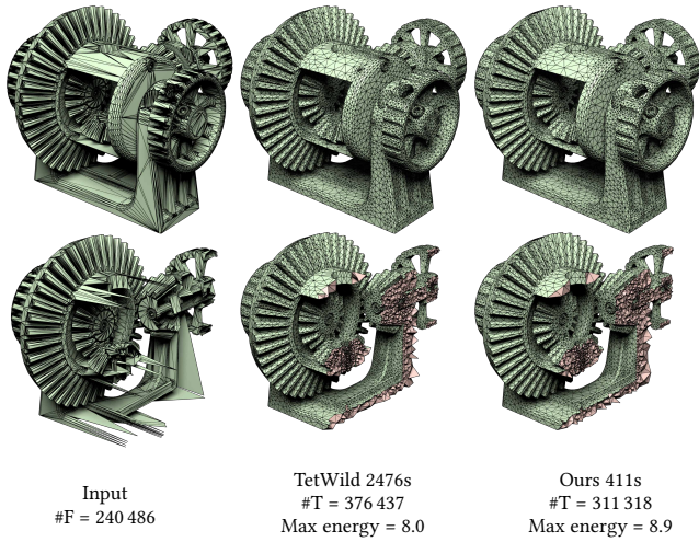
Fig. 16. Our method (right) produces high-quality tet-meshes that are similar to TetWild (middle).
