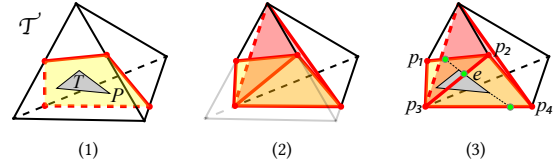
Fig. 29. Example for preserving an open-boundary edge e of triangle T . (1) Insert T and \mathcal{T}_{\bar{T}} = \{T\} in this case. (2) The sub-tetrahedra of \mathcal{T} after subdivision. (Only sub-tetrahedra behind T are shown for better visualization.) (3) Inserting edge e and get the intersection points (in green).
