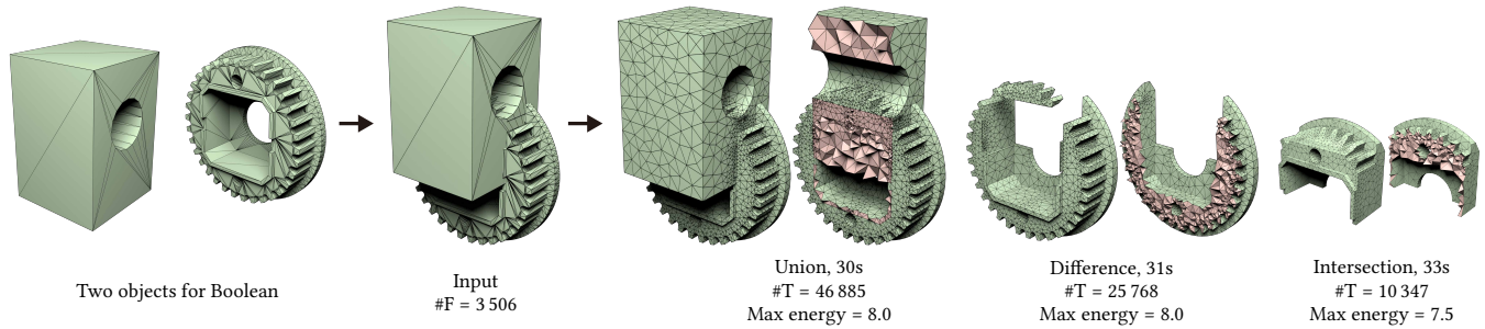
Fig. 23. Three Boolean operations computed on non-manifold, self-intersecting, and non-PWN input surface meshes. The left are two objects for Boolean operation. The middle is the input surface mesh of FTETWILD. The right are our output meshes after computing the union, difference, and intersection between the two objects. The average max AMIPS energy of outputs and average time of different operations are with small variance.
