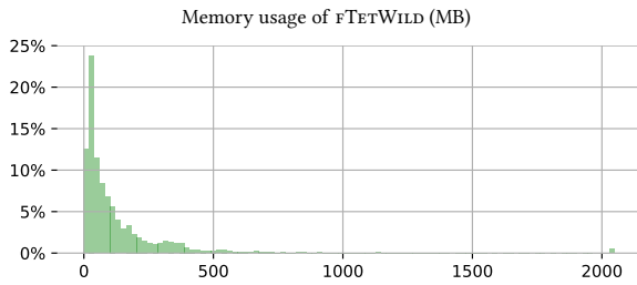
Fig. 13. Histogram of memory usage of fTetWild over the Thingi10k dataset (data truncated at 2GB).
