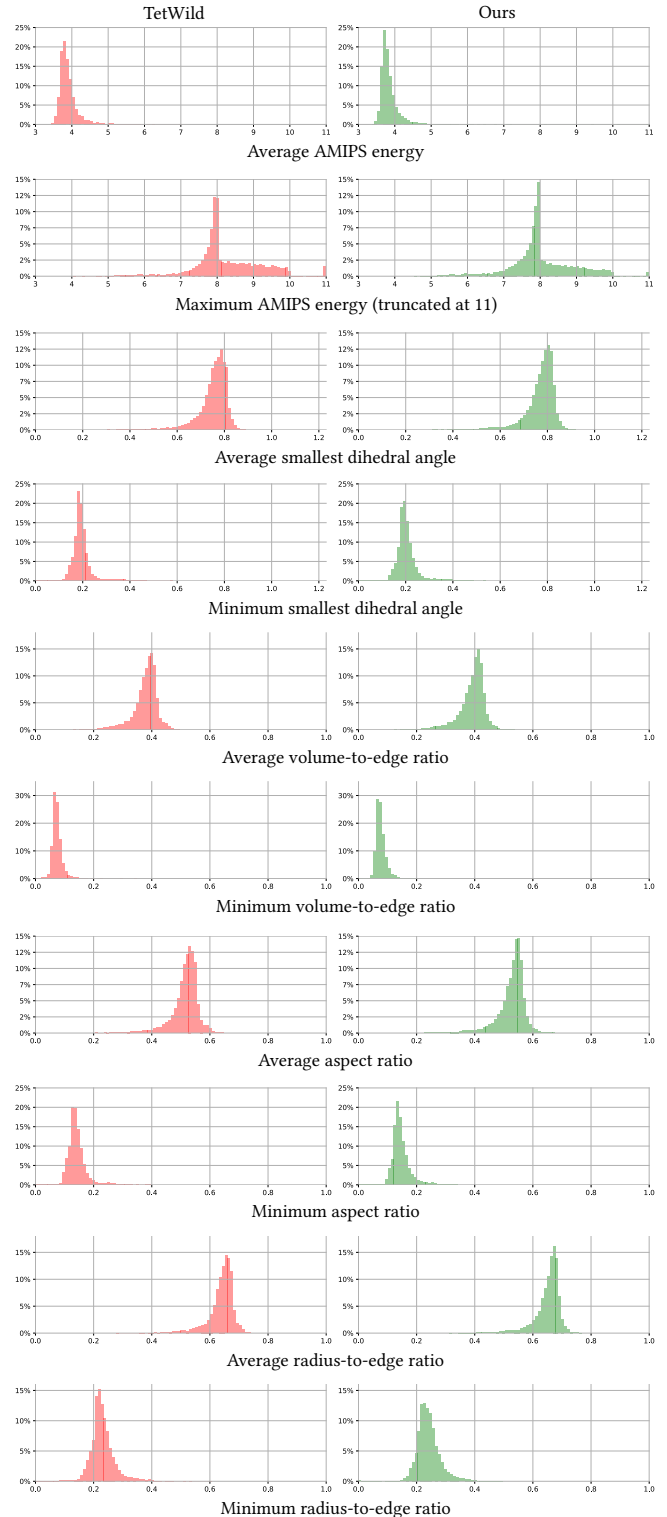
Fig. 17. Histogram for mesh quality comparison of TetWild (red) and our method (green) in five different quality measures. The statistic is based on the output of the whole Thingi10k dataset.
