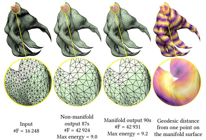
Fig. 20. Example of a non-manifold surface mesh (left) which is automatically repaired by our algorithm (right second).
