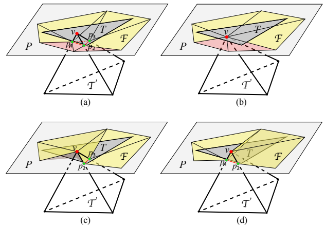
Fig. 7. Plane P intersects \mathcal{T}_I ( \mathcal{T} \in \mathcal{T}_I ). (a) The faces of \mathcal{F} (marked in yellow) are the covering of triangle T . (b) Snapping v to its closest point on P and expanding \mathcal{F} to include red triangles makes \mathcal{F} safely covering T . (c) Snapping a boundary vertex p_1 of \mathcal{F} to v changes the area of \mathcal{F} and make it not covering T . (d) Snapping an interior vertex p_3 of \mathcal{F} to v does not change the boundary of \mathcal{F} : \mathcal{F} is still covering T .
