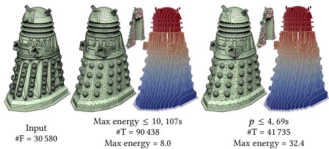
Fig. 26. Two different stopping criteria of our algorithm. The full optimization (middle) improves the mesh to high quality, while using the criterion in [Schneider et al. 2018] (right) results in lower mesh quality but faster meshing and smaller mesh size. The color shows the solution of the volumetric Laplace equation.
