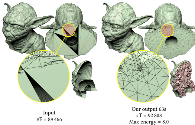
Fig. 2. Example of an input surface mesh with self-intersections and a bad triangulation on the base. \text{FTETWILD} converts this model into a high-quality tetrahedral mesh.
