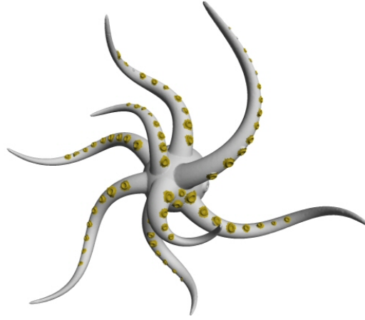
Fig. 10. Self similarity. The suction cups on the tentacle of the octopus model have a similar shape. Note that their size varies across the model.
