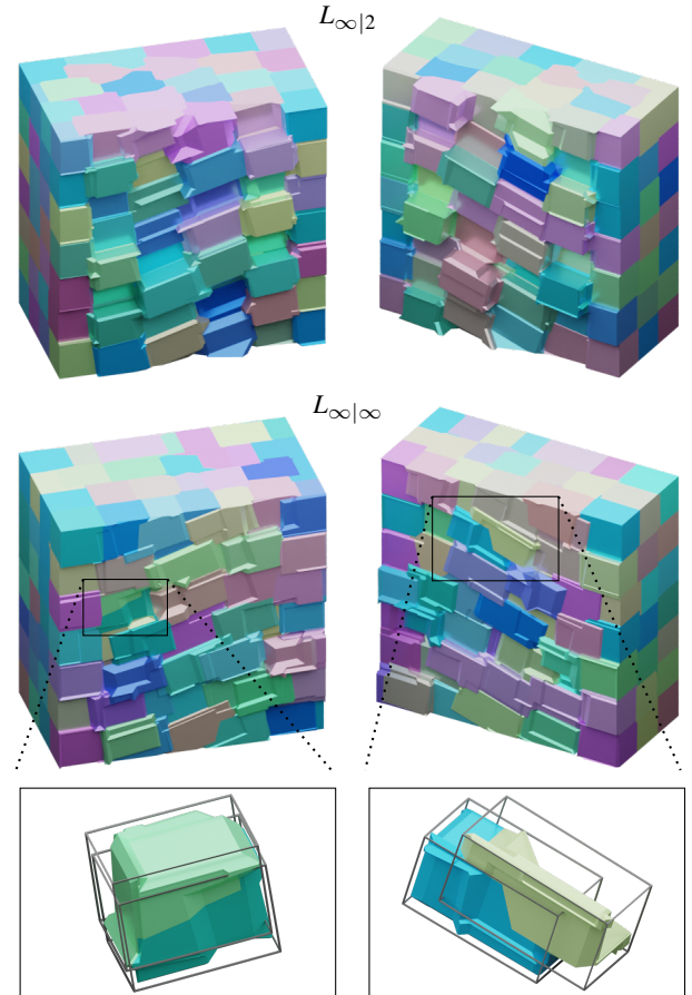
Figure 22: Anisotropic 3D CVTs with different cell / centroid combinations. The isolated L_{\infty|\infty} cells have largely overlapping bounding-boxes (bottom), thus very close centroids (Section 6.1).
