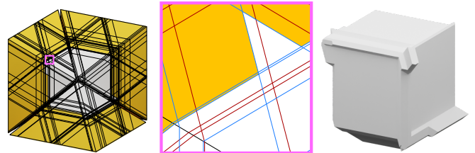
Figure 10: The cut & clip algorithm on the initialization pyramids. The exposed inner of a cell (left) shows only the \{-\mathbf{x}, +\mathbf{y}, -\mathbf{z}\} pyramids with their cuts. Clipped geometry is highlighted in yellow. Valid and invalid cuts are marked in the zoom-in (center). The eventually extracted geometry for the L_\infty cell is shown on the right.
