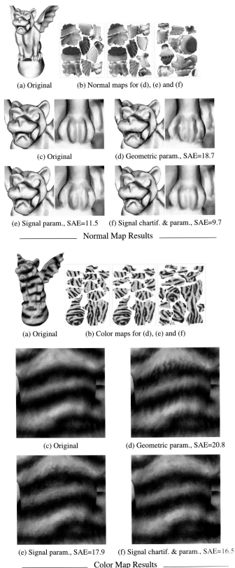
Figure 8: Signal-specialized atlas results (256 × 256 maps).
