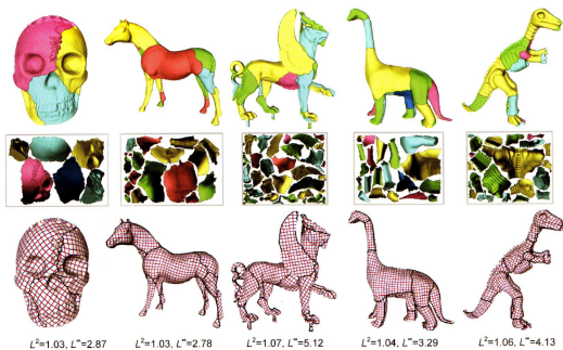
Plate 1: Chartification and parameterization results produced by our algorithm. The top row shows the charts on the 3D surface, the middle row shows the texture atlases, the bottom row shows iso-parameter lines over the surfaces.
