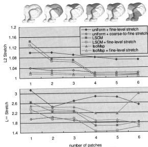
Figure 3: Stretch vs. number of patches for different parameterizations.
