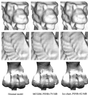
Figure 7: Comparison of geometry remeshing methods. Geometry images have resolution 256 × 256.
